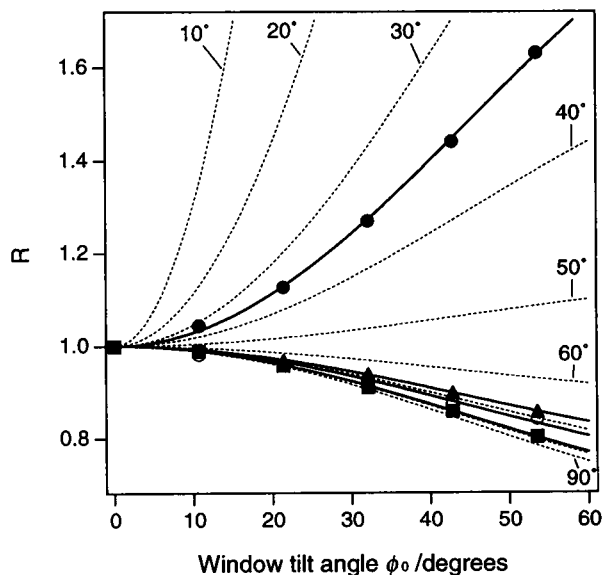
FIGURE 2 R versus \phi_0 plots for the bands at 1761 \text{cm}^{-1} (●), 1527 \text{cm}^{-1} (○), 1202 \text{cm}^{-1} (■), and 1169 \text{cm}^{-1} (▲). The bands at 1527, 1202, and 1169 \text{cm}^{-1} are not included in Fig. 1. The points were fitted with Eq. 2 by the least-squares method. The fitted curves are shown by thick lines. Dotted lines show the theoretical lines according to Eq. 2 from \theta_0 = 10 – 90^\circ . The line at \theta_0 = 10^\circ has the largest slope. The slope decreases with the increment of the angle of \theta_0 and becomes negative above 54.7^\circ (magic angle).
