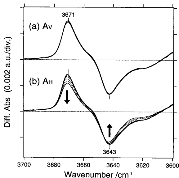
FIGURE 3 Changes of the M minus BR spectra in the 3700–3600 \text{cm}^{-1} region with the tilting of the sample window for the A_V (a) and A_H (b) components. The thick solid lines are the spectra at \phi_0 = 0^\circ ; the dotted lines are those at \phi_0 = 10.7, 21.4, 32.1 and 42.8^\circ ; the thin solid line is that at \phi_0 = 53.5^\circ . Arrows indicate the direction for the spectral changes with the tilting.
