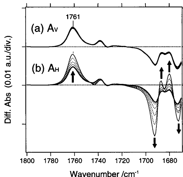
FIGURE 1 Changes of the M minus BR spectra in the 1800–1670 \text{cm}^{-1} region with the tilting of the sample window for the A_V (a) and A_H (b) components. The thick solid lines are the spectra at \phi_0 = 0^\circ ; the dotted lines are those at \phi_0 = 10.7, 21.4, 32.1 , and 42.8^\circ ; and the solid thin lines are those at \phi_0 = 53.5^\circ . Arrows indicate the direction for the spectral changes with the tilting.
